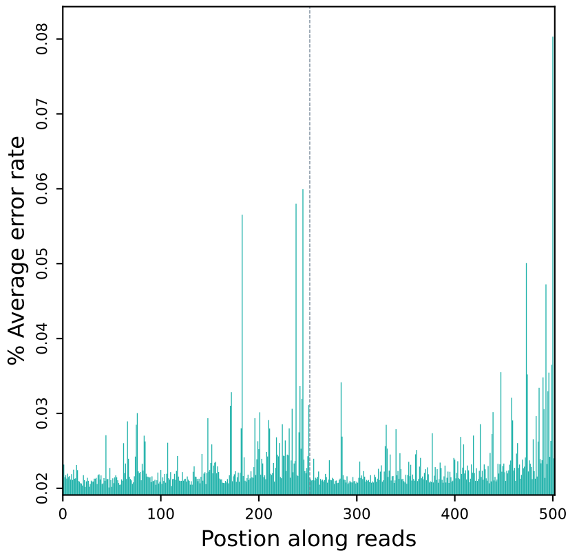
Error rate distribution along reads (R10803)
